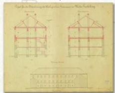
Draft of part of the monastery in Siroki Brijeg, planned for the theological seminar, 1909. (ABH, ZVS, 5-33/1901)
